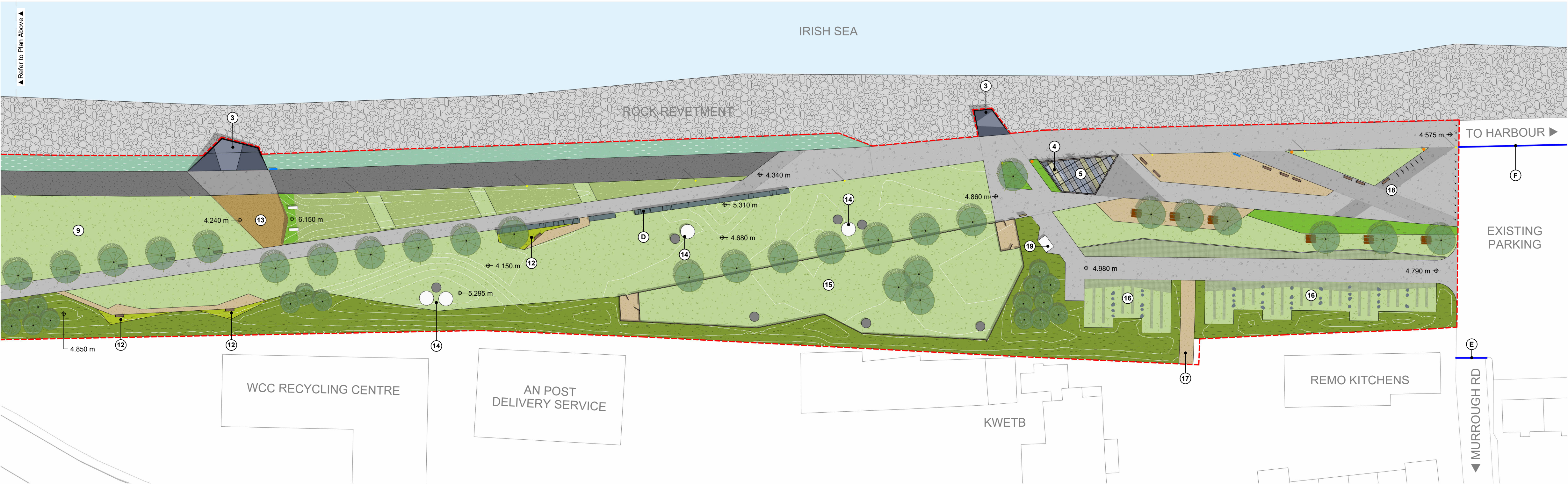
2 South Landscape Layout SCALE - 1 : 500
